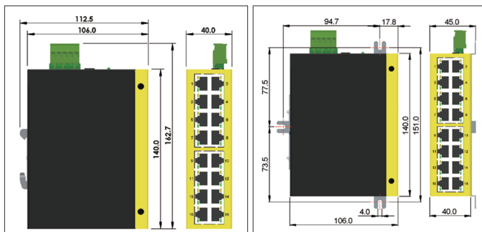
DIN-Rail Mounting Dimension
