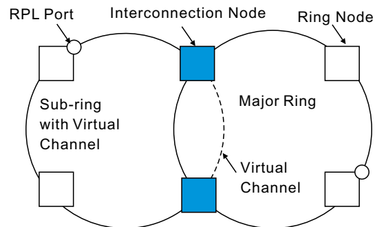
Figure 323: Sub-ring with Virtual Channel
