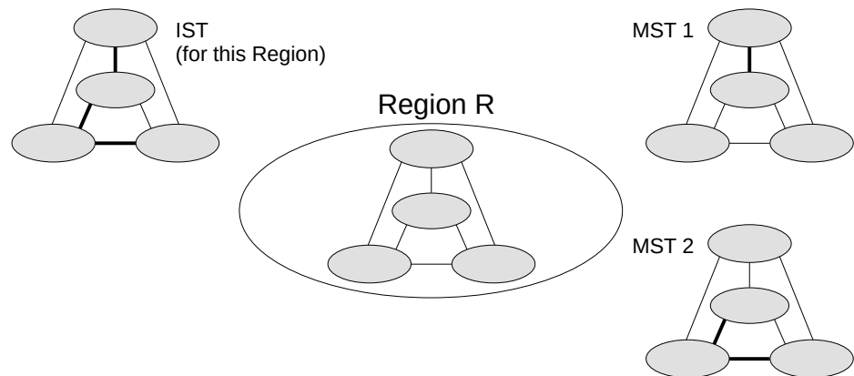
Figure 121: MSTP Region, Internal Spanning Tree, Multiple Spanning Tree
