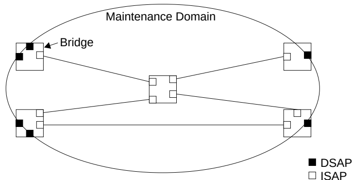
Figure 334: Single CFM Maintenance Domain
