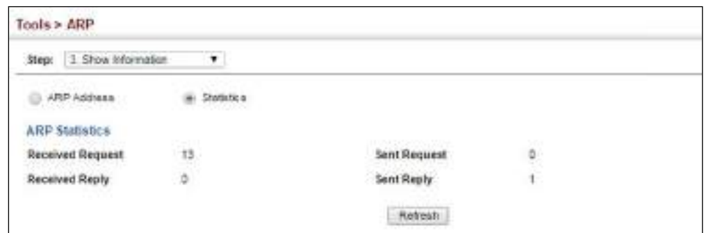
Figure 457: Displaying ARP Statistics
