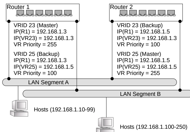
Figure 514: Several Virtual Master Routers Configured for Mutual Backup and Load Sharing
