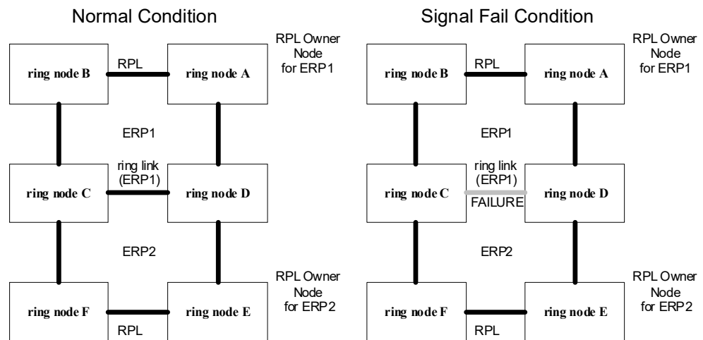
Figure 319: Ring Interconnection Architecture (Multi-ring/Ladder Network)
