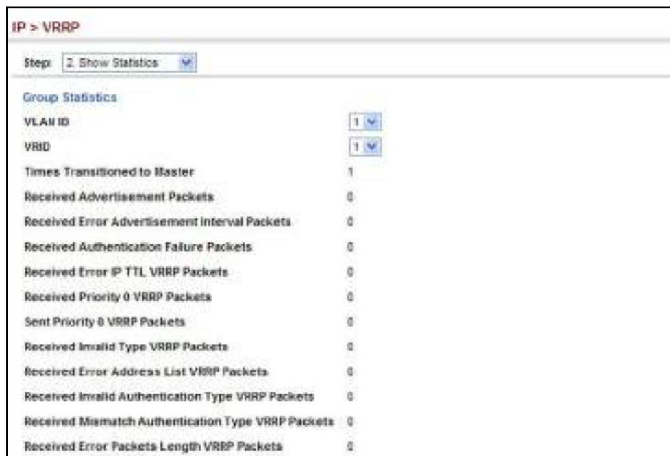
Figure 521: Showing Counters for Errors Found in a VRRP Group
