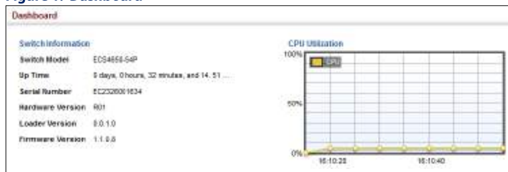
Figure 1: Dashboard
