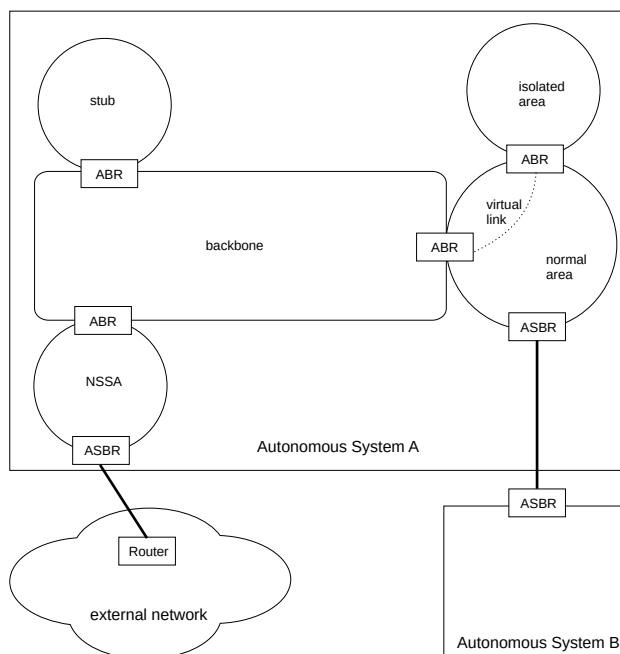
Figure 540: Configuring OSPF
