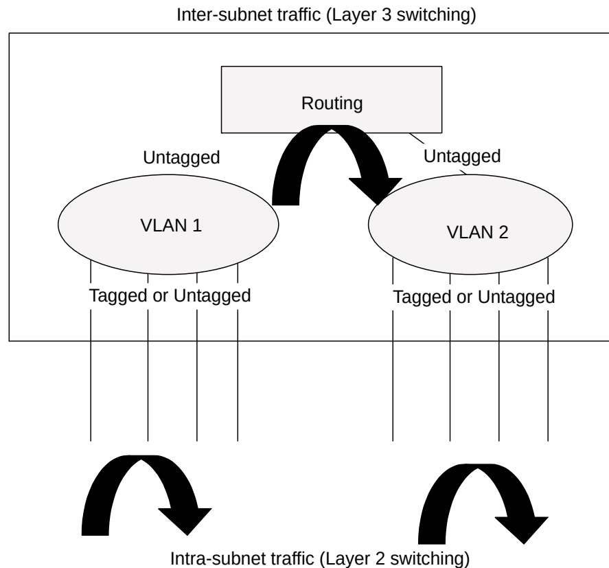
Figure 473: Virtual Interfaces and Layer 3 Routing
