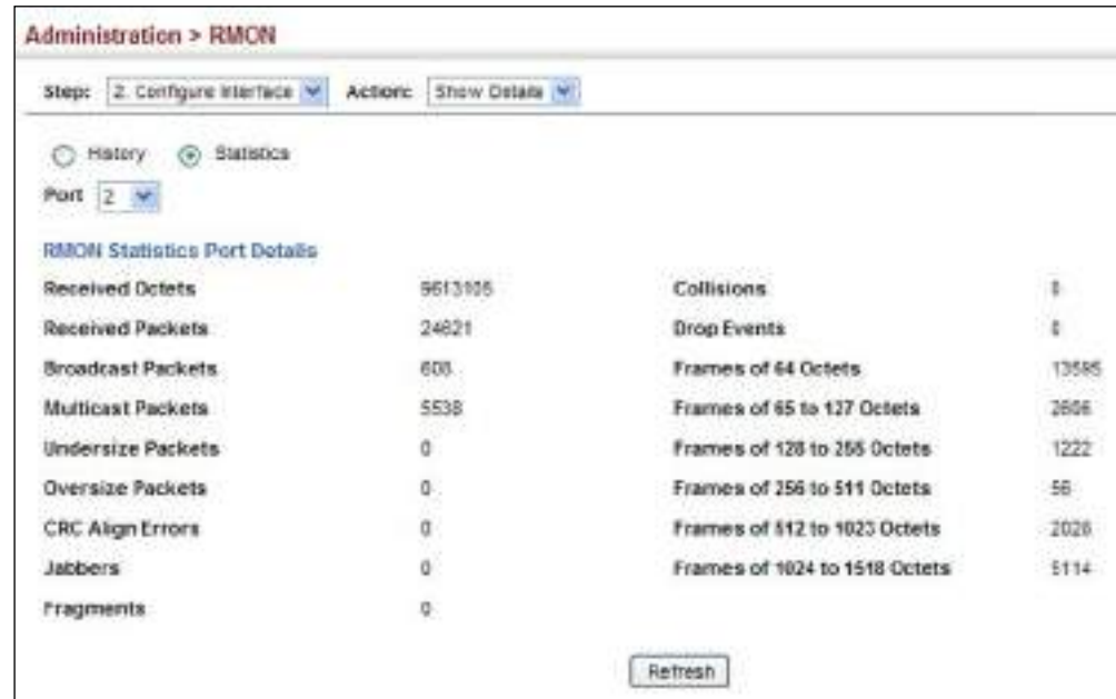
Figure 308: Showing Collected RMON Statistical Samples
