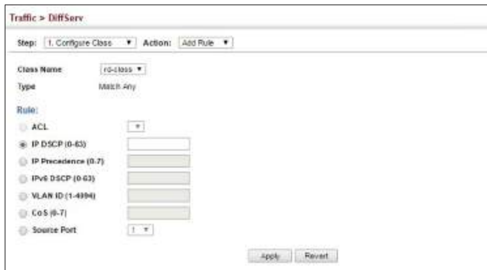
Figure 161: Adding Rules to a Class Map
