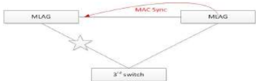
Figure 332: MLAG Peer Operation
