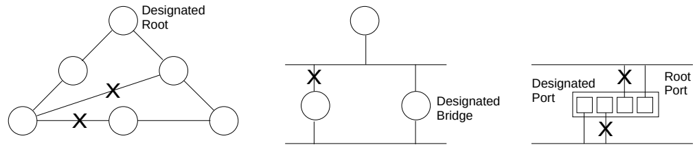
Figure 120: STP Root Ports and Designated Ports
