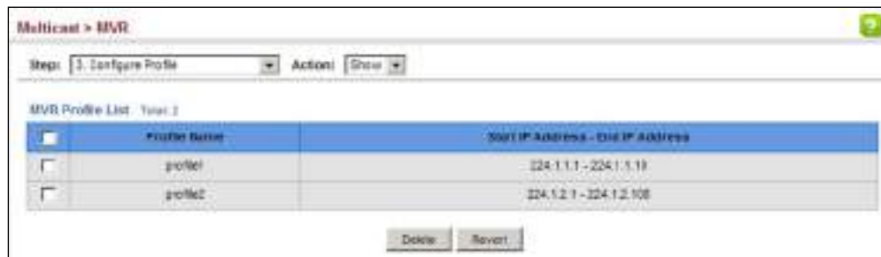
Figure 426: Displaying MVR Group Address Profiles
