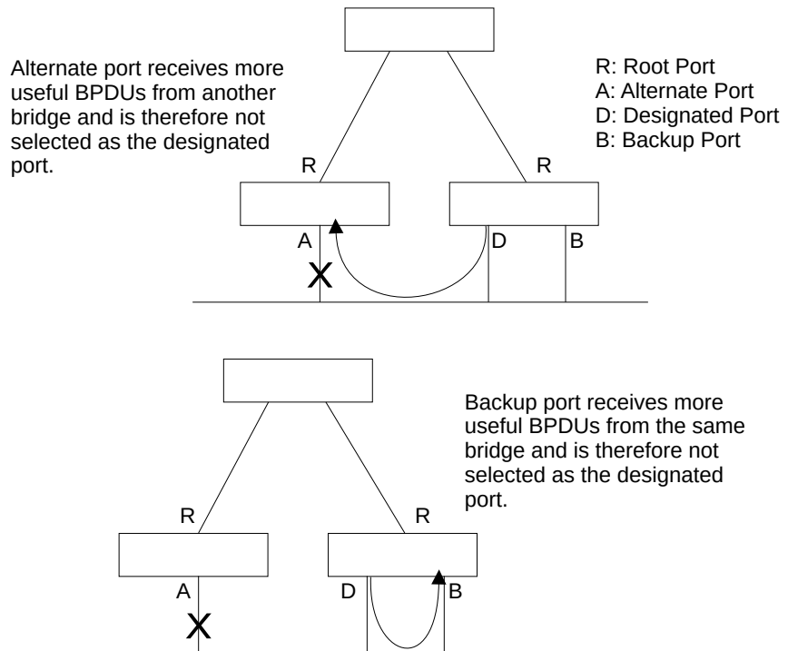
Figure 130: STA Port Roles
