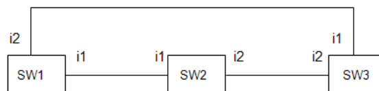
Figure 128: Determining the Root Port
