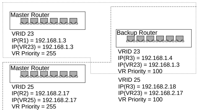
Figure 514: Several Virtual Master Routers Configured for Mutual Backup and Load Sharing
