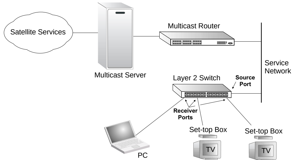
Figure 422: MVR Concept
