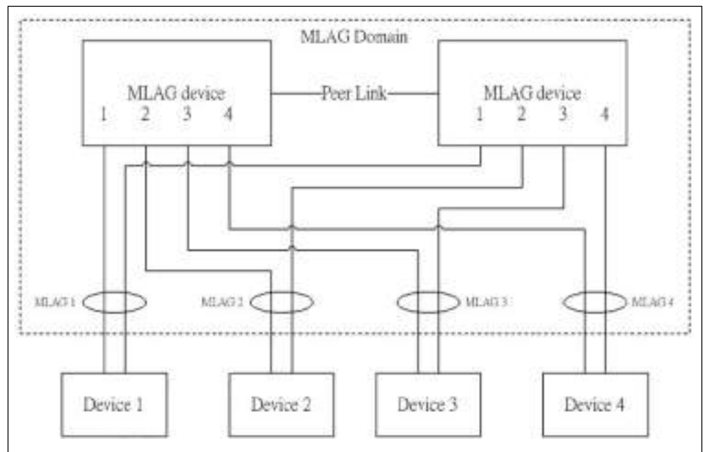
Figure 329: MLAG Domain Topology
