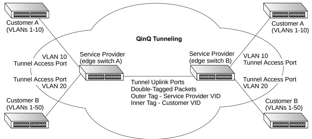
Figure 90: QinQ Operational Concept
