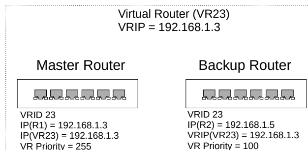
Figure 512: Master Virtual Router with Backup Routers
