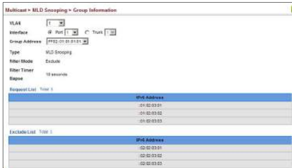
Figure 404: Showing IPv6 Multicast Services and Corresponding Sources
