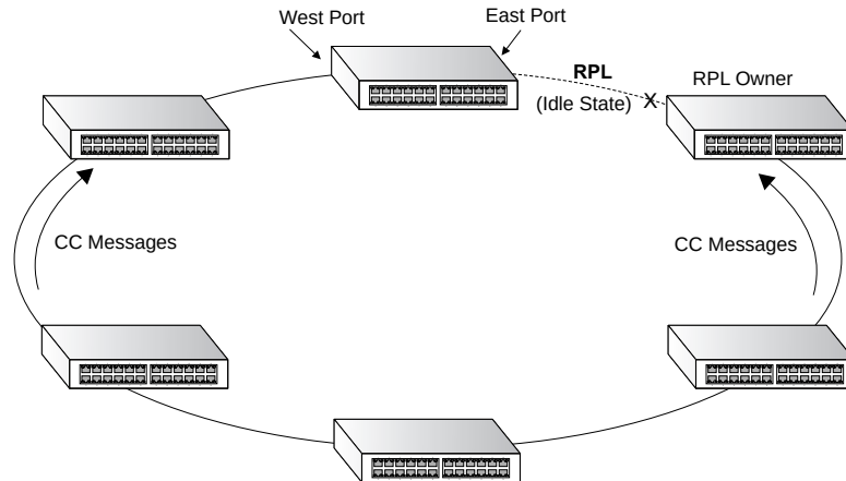
Figure 318: ERPS Ring Components
