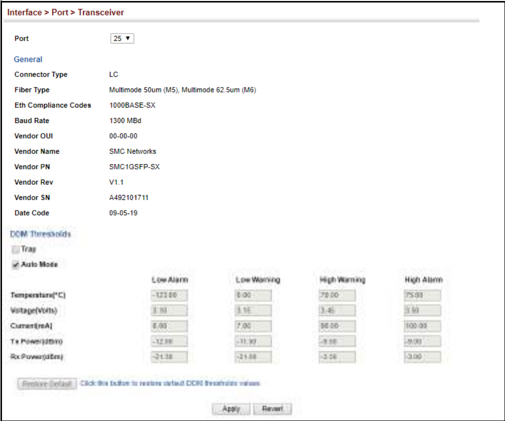
Figure 42: Displaying Transceiver Data
