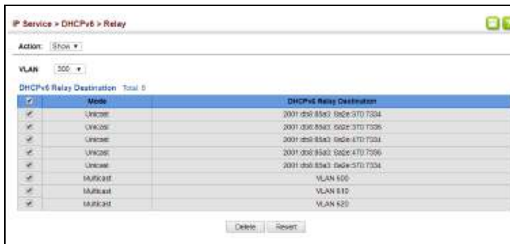
Figure 367: Enabling DHCPv6 Relay Agent for Multicast mode.
