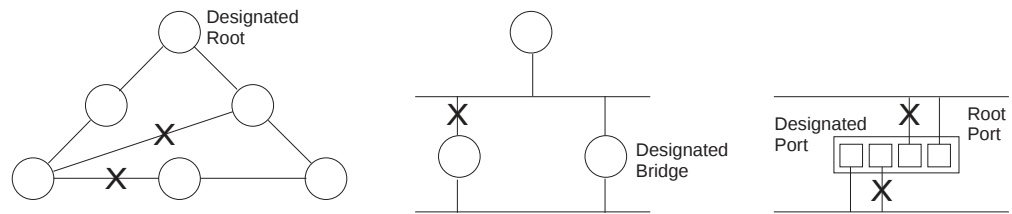
Figure 94: STP Root Ports and Designated Ports
