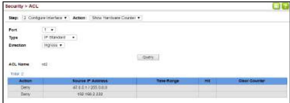
Figure 179: Showing ACL Statistics
