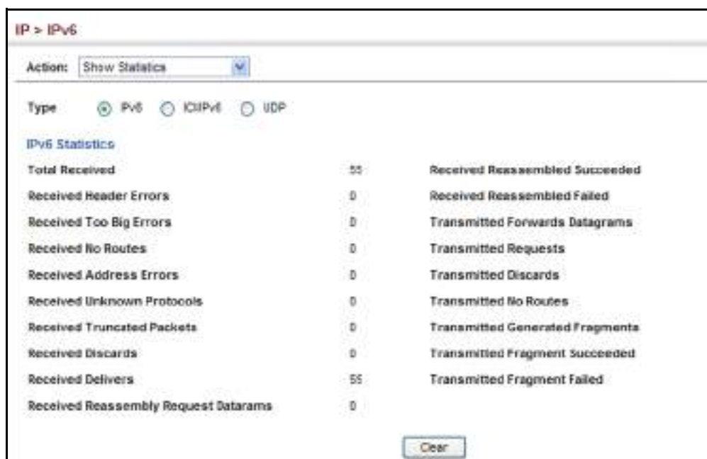
Figure 324: Showing IPv6 Statistics (IPv6)
