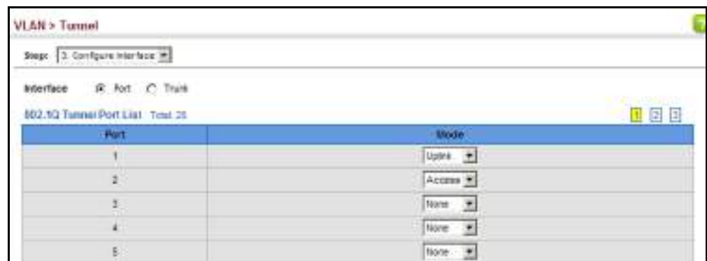
Figure 81: Adding an Interface to a QinQ Tunnel
