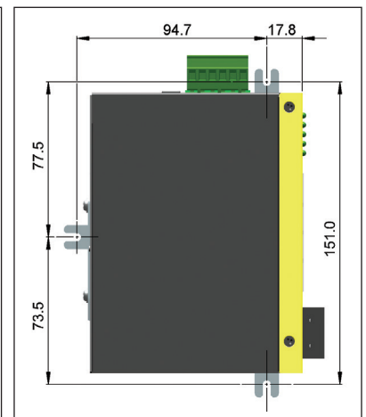
Panel Dimension
