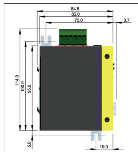
Panel Dimension
