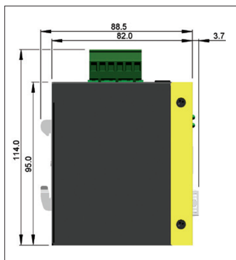
DIN-Rail Dimension
