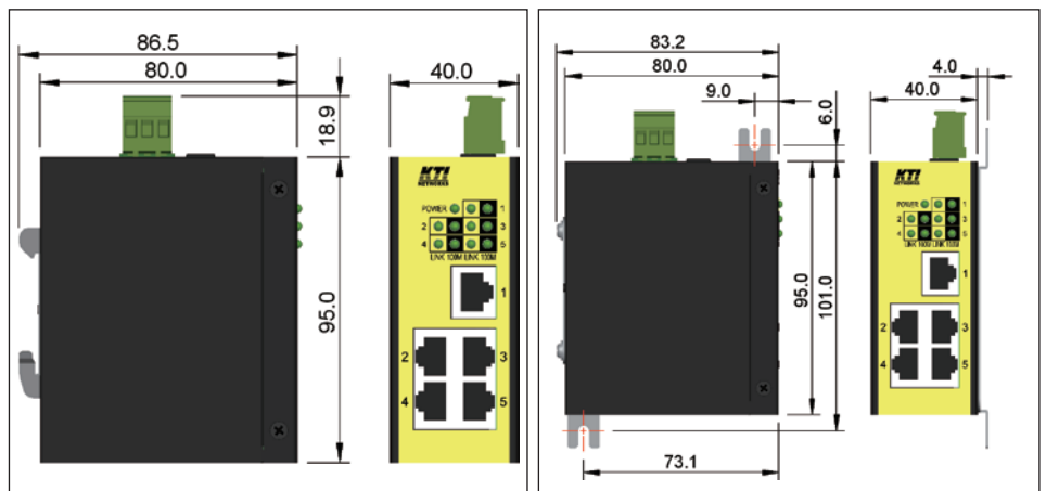
DIN-Rail Dimension
